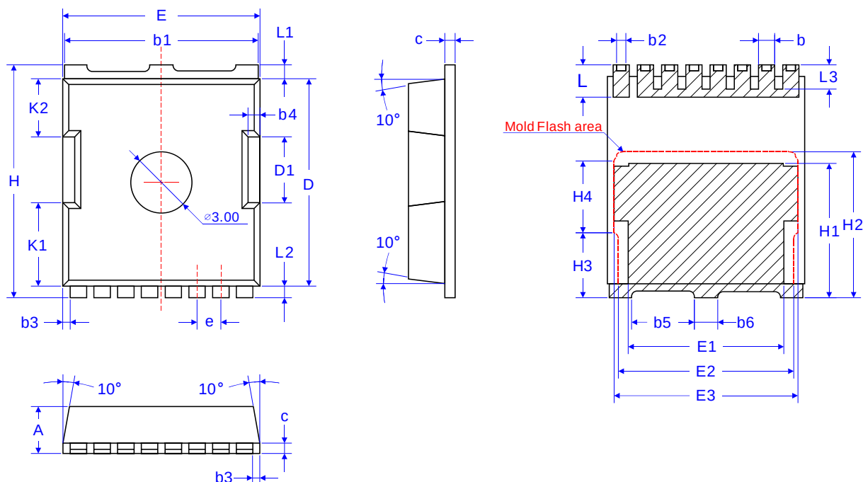
TOLL-8L Package
