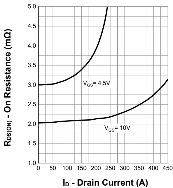
On Resistance
