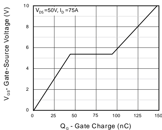
Figure 12. Gate Charge
