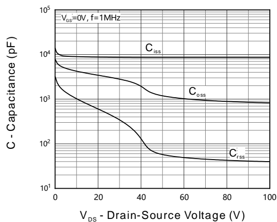
Figure 11. Capacitance
