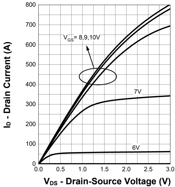
Output Characteristics
