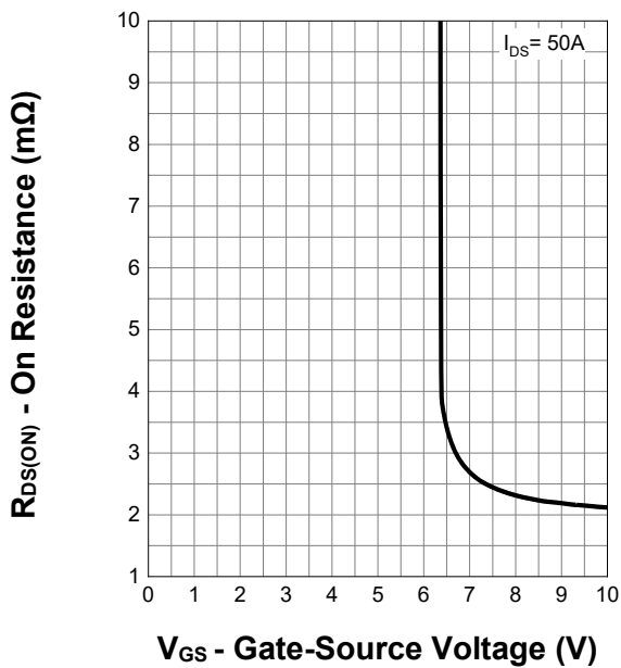
Transfer Characteristics
