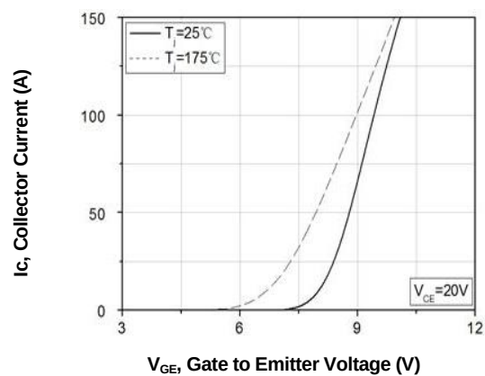
Figure 6. Typical transfer characteristic ( V_{CE}=20V )
