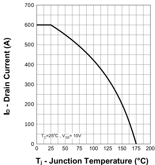
Current Capability
