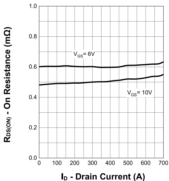
On Resistance
