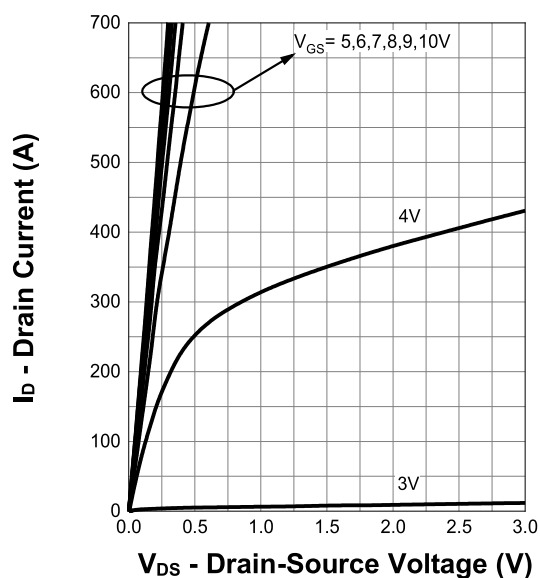
Output Characteristics
