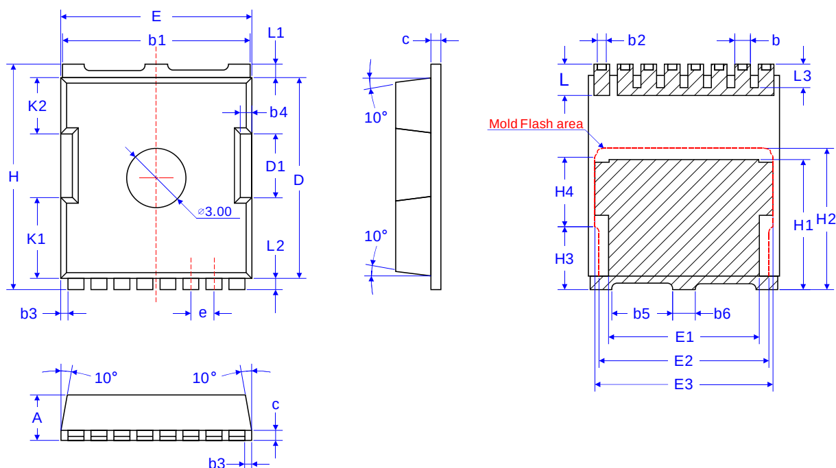
TOLL-8L Package
