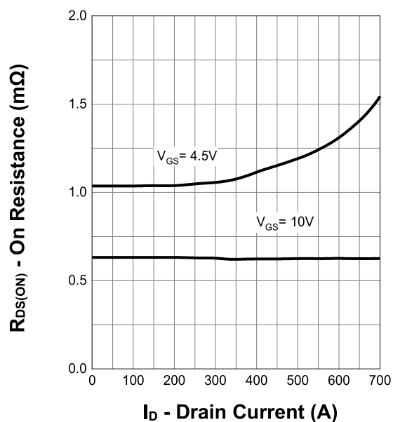
On Resistance
