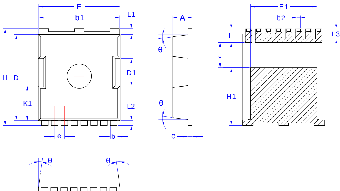
TOLL-8L Package
