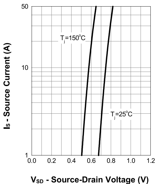
Diode Forward Current
