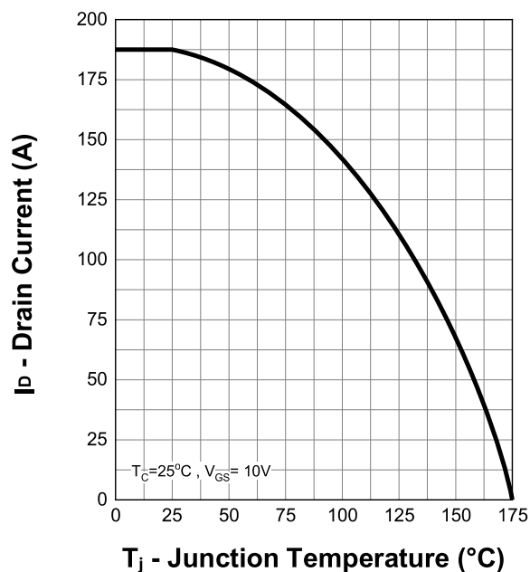
Current Capability
