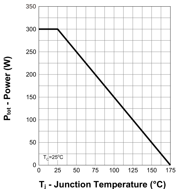
Power Capability
