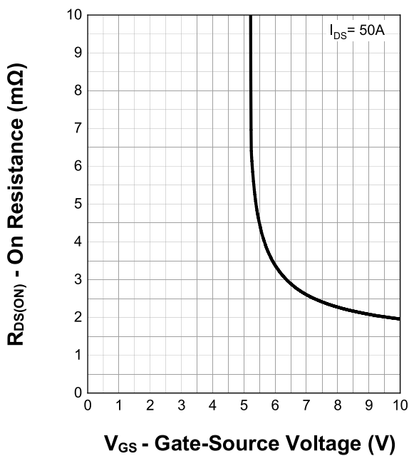
Transfer Characteristics
