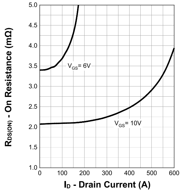
On Resistance
