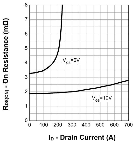
On Resistance
