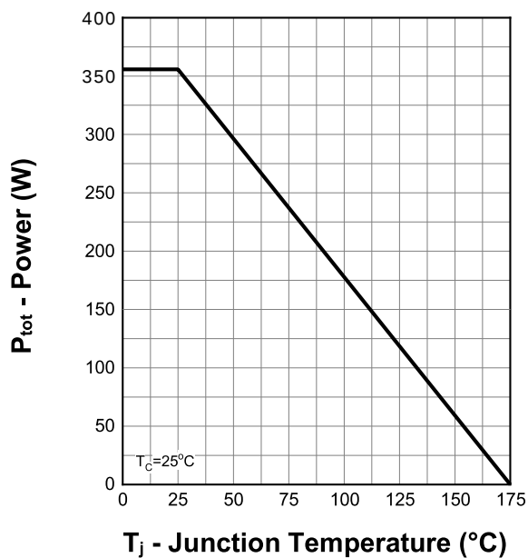
Power Capability
