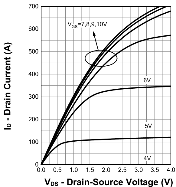
Output Characteristics
