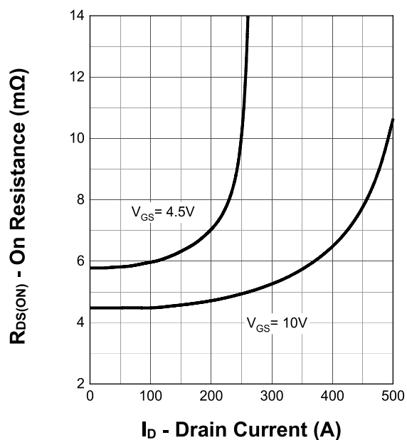
On Resistance
