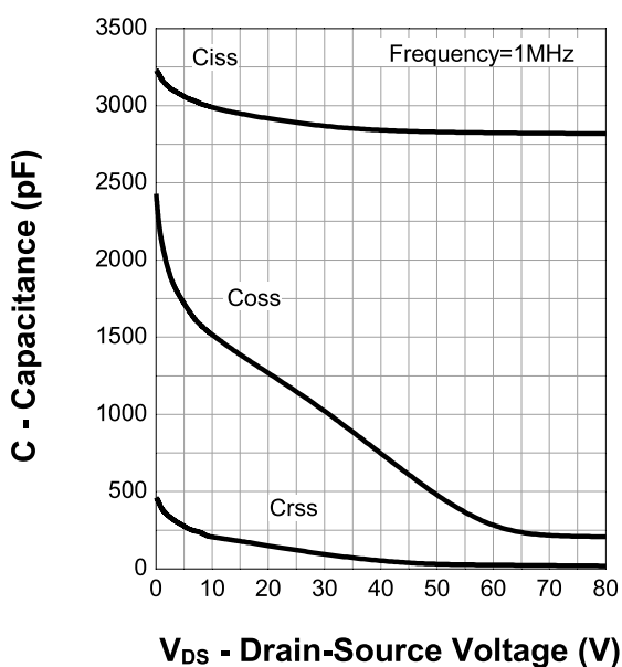
Capacitance
