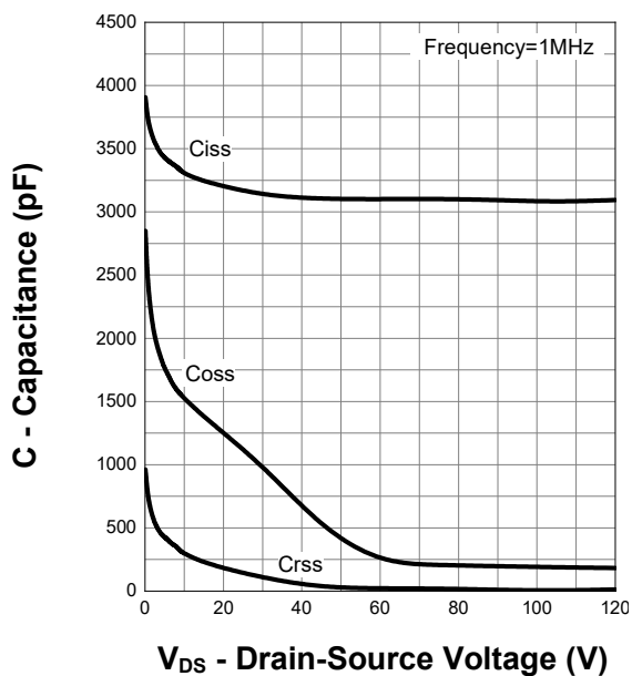
Capacitance
