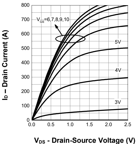
Output Characteristics
