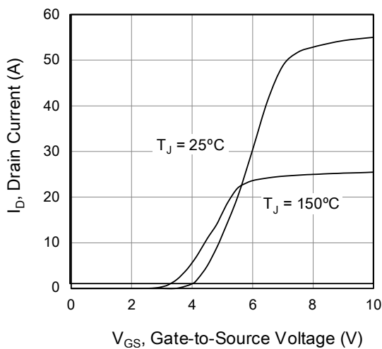
Figure 5: Transfer Characteristics
