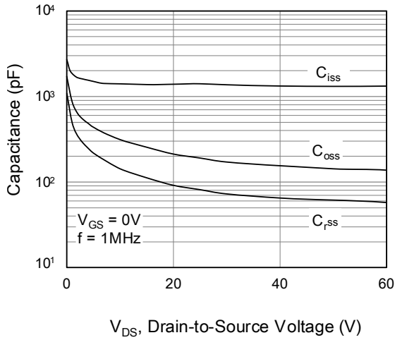
Figure 7: Capacitance
