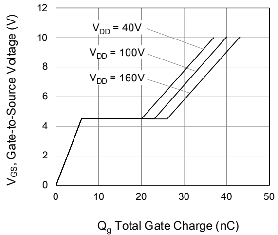
Figure 8: Gate Charge
