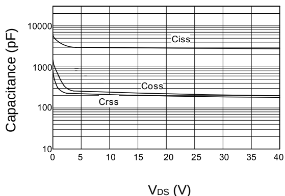
Figure 11. Capacitance
