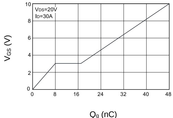
Figure 12. Gate charge
