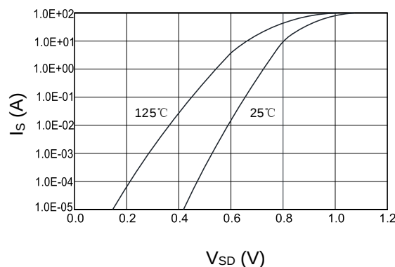
Figure 10. Forward characteristics of body diode
