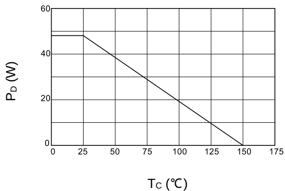
Figure 1. Power Capability
