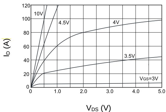
Figure 3. Output characteristics
