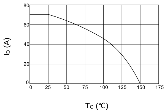
Figure 2. Current Capability
