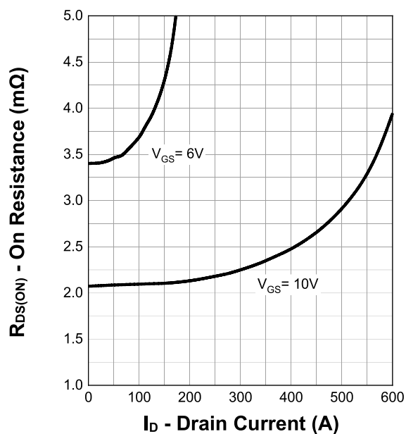
On Resistance
