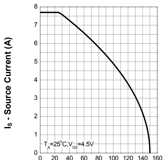
Source Current
