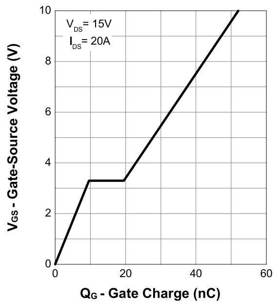
Gate Charge
