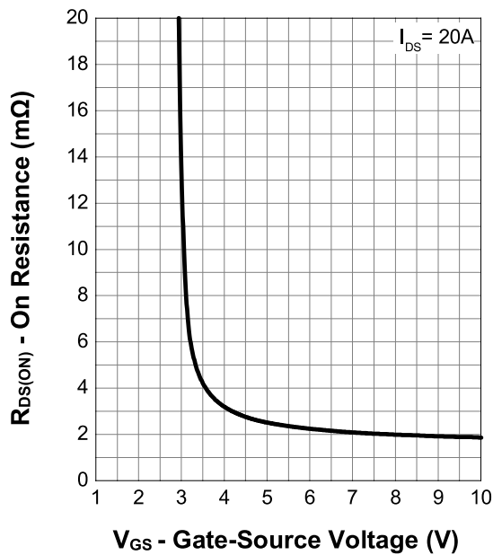
Transfer Characteristics
