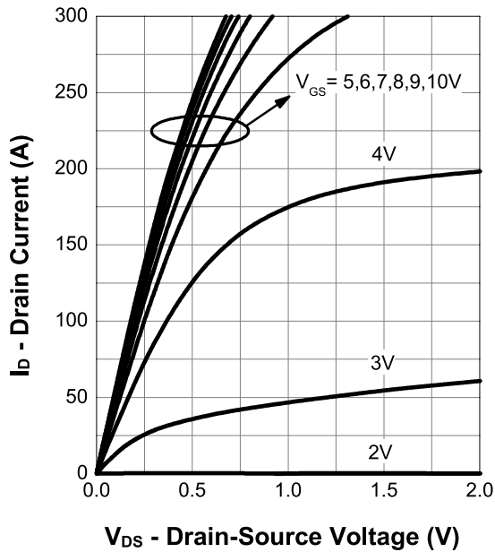
Output Characteristics
