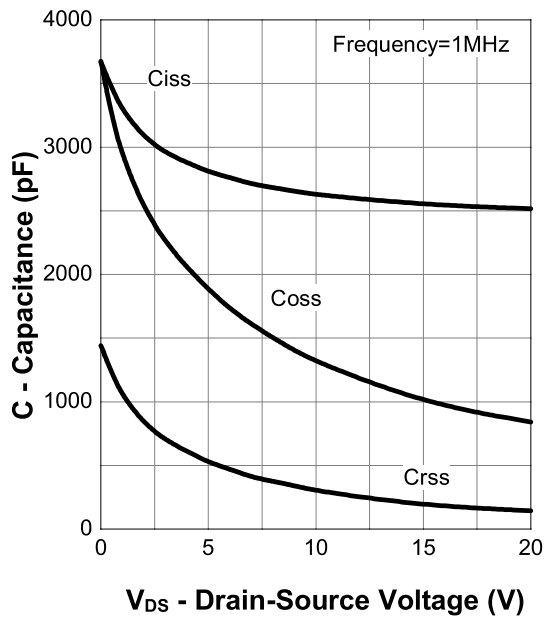
Capacitance
