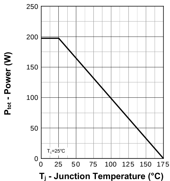
Power Capability
