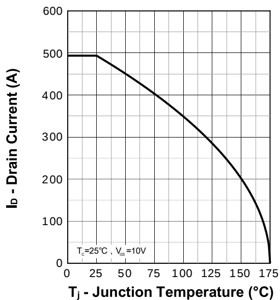
Current Capability
