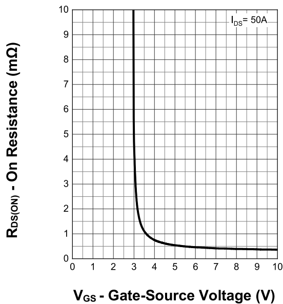
Transfer Characteristics
