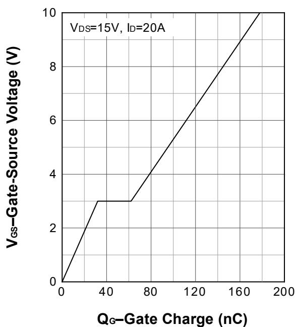
Gate Charge
