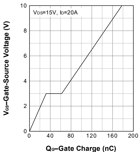
Gate Charge
