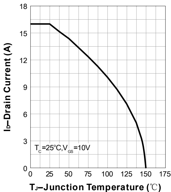
Current Capability
