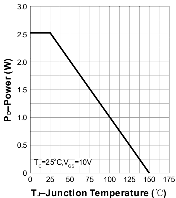
Power Capability
