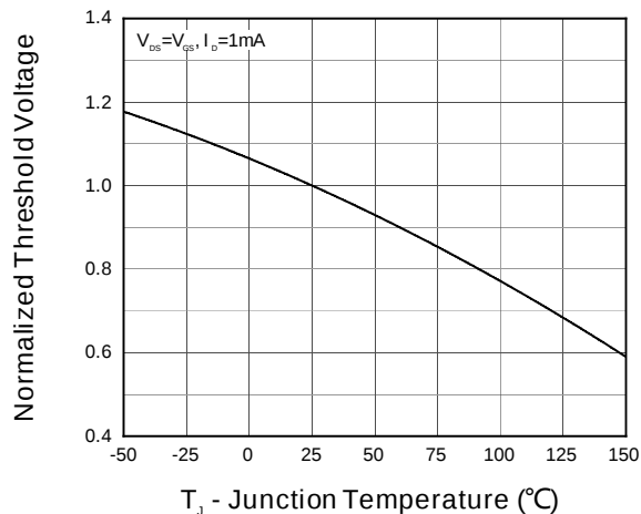
Figure 8. Normalized V_{GS(th)}
