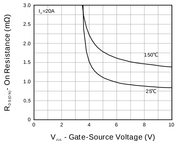
Figure 7. Transfer Characteristics
