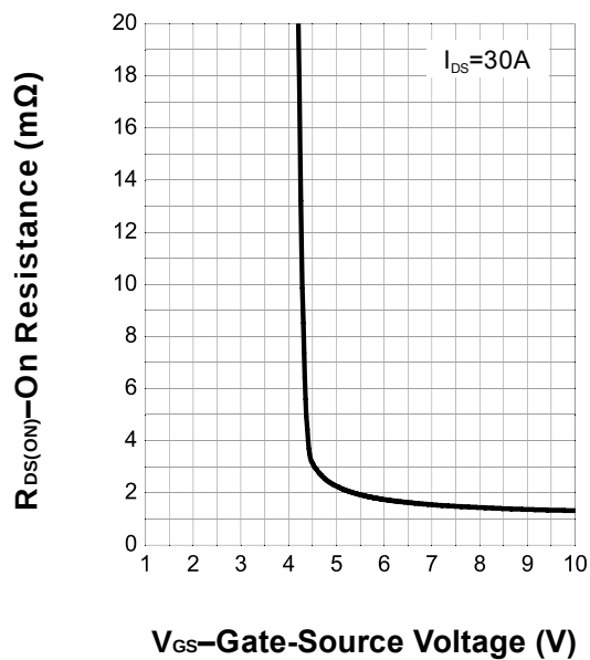
Transfer Characteristics
