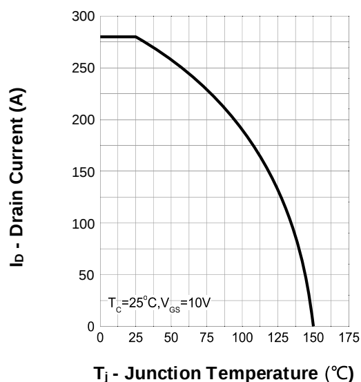
Current Capability
