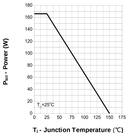
Power Capability
