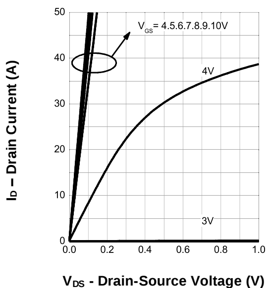
Output Characteristics
