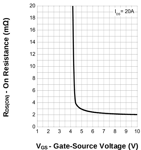
Transfer Characteristics
