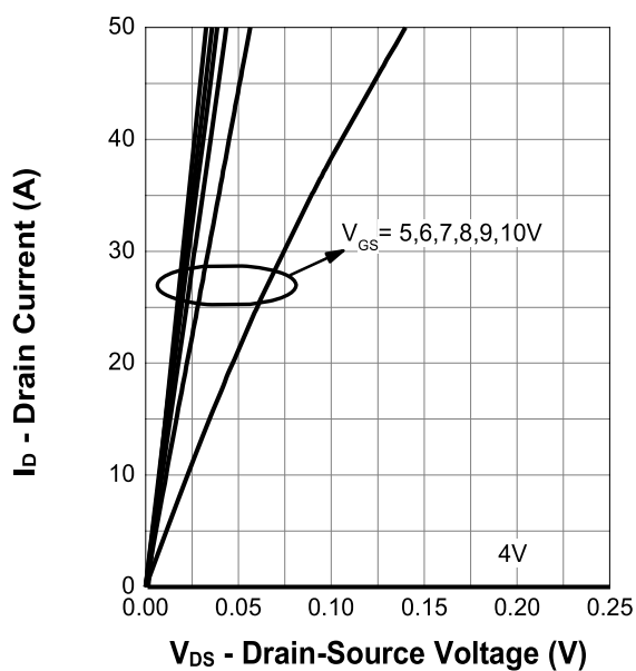
Output Characteristics
