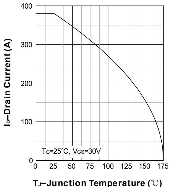
Current Capability
