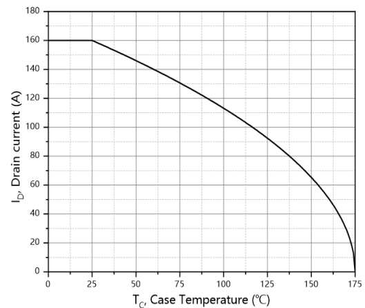
Figure 10. Drain current
