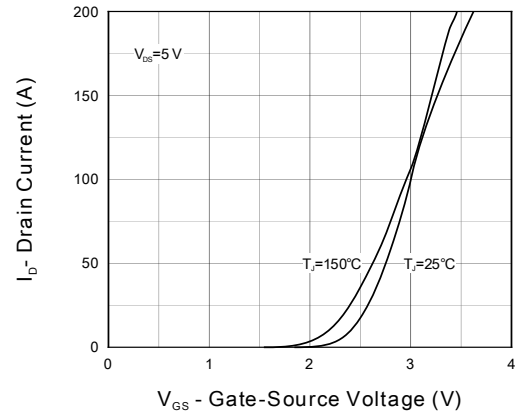
Figure 8. Transfer Characteristics
