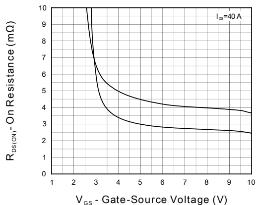
Figure 7. R_{DS(ON)} vs. V_{GS}
