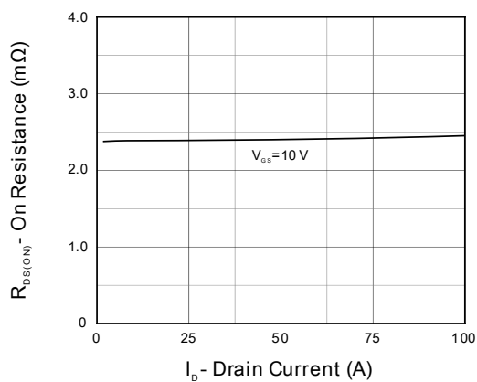
Figure 6. On Resistance
