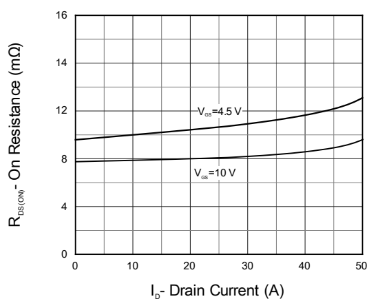
Figure 6. On Resistance
