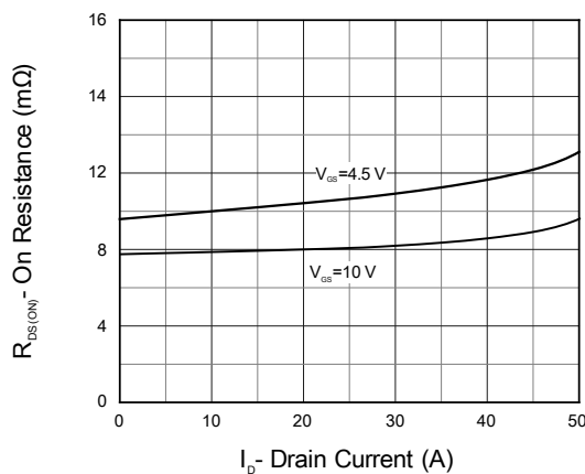
Figure 6. On Resistance
