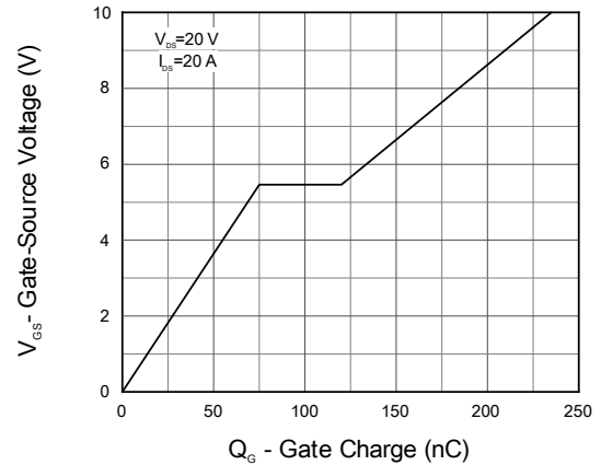
Figure 12. Gate Charge
