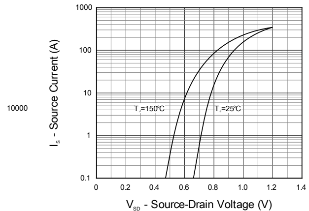
Figure 10. Diode Forward Current
