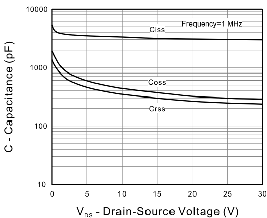
Figure 11. Capacitance
