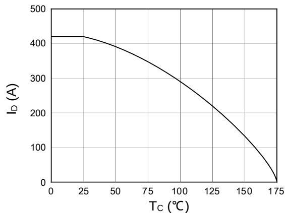
Figure 2. Current Capability
