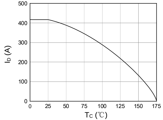
Figure 2. Current Capability
