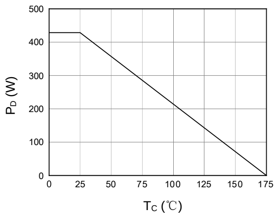
Figure 1. Power Capability
