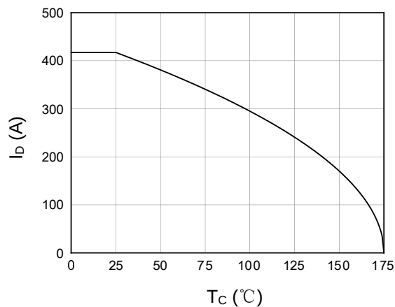
Figure 2. Current Capability
