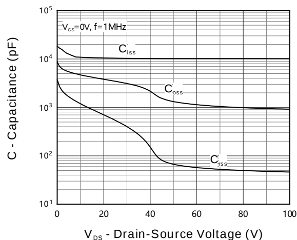
Figure 11. Capacitance
