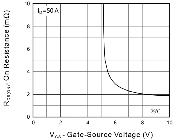
Figure 7. Transfer Characteristics
