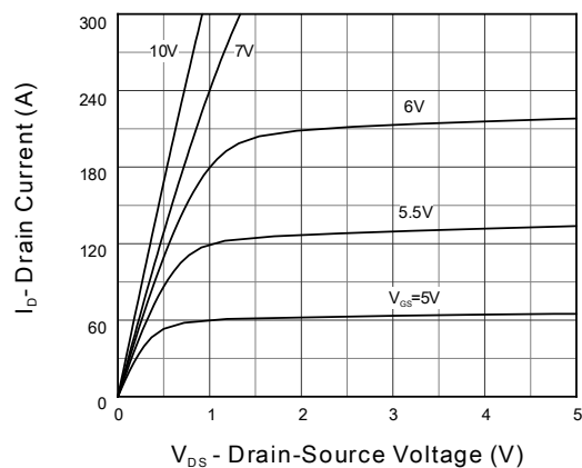
Figure 5. Output Characteristics
