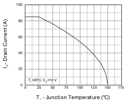
Figure 2. Current Capability
