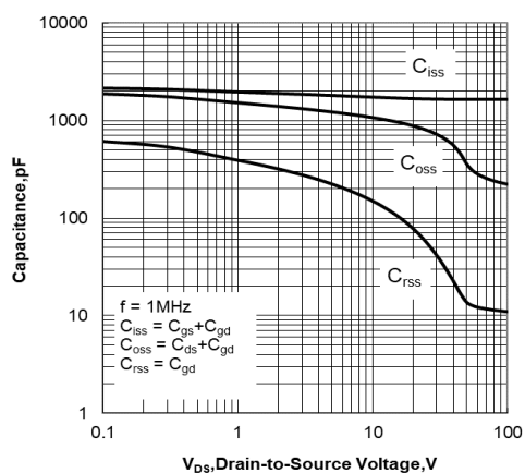
Figure 5. Capacitance Characteristics
