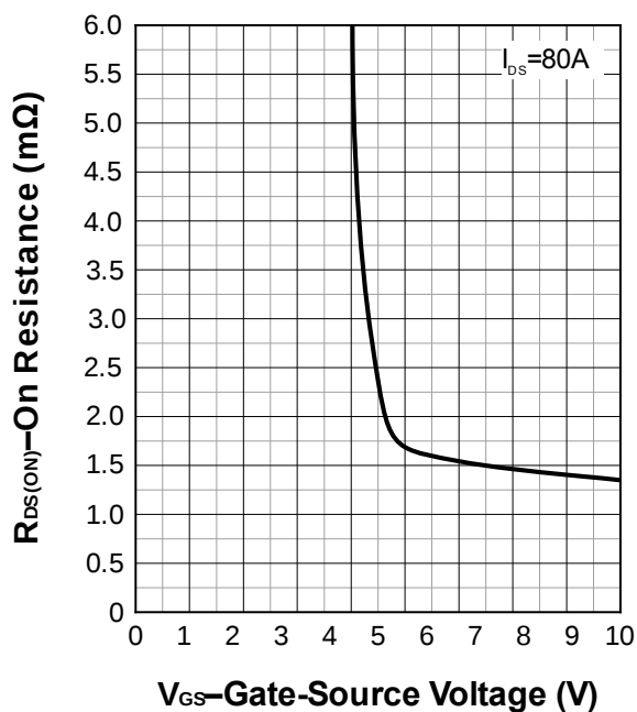
Transfer Characteristics
