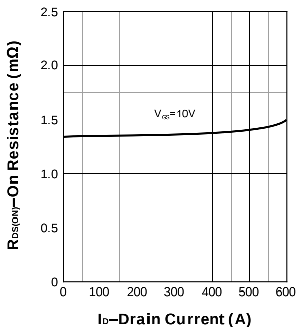
On Resistance
