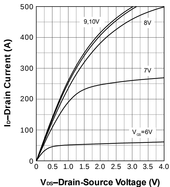
Output Characteristics
