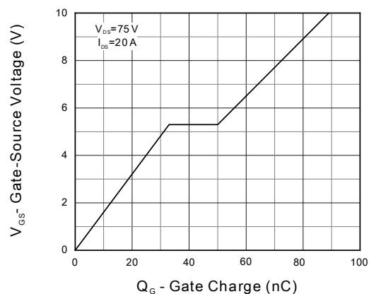
Figure 12. Gate Charge
