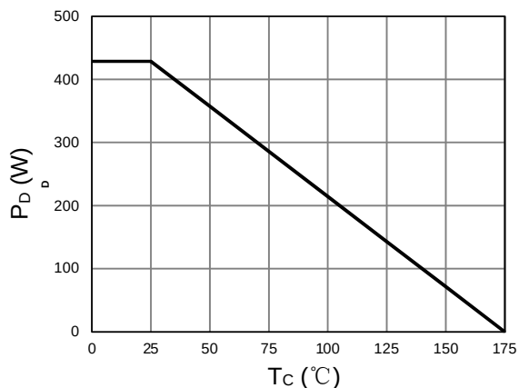
Figure 1. Power Capability
