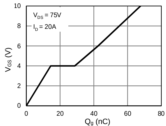
Figure 12. Gate charge
