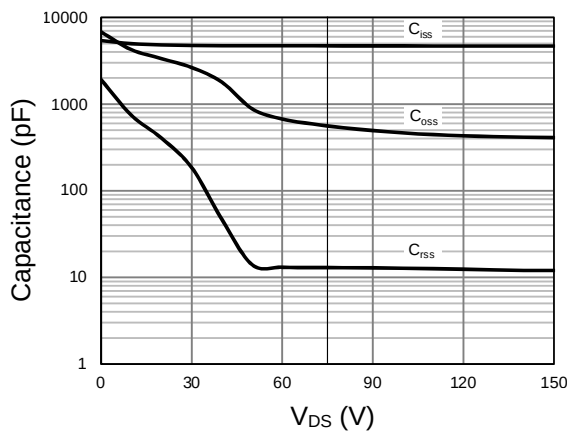
Figure 11. Capacitance
